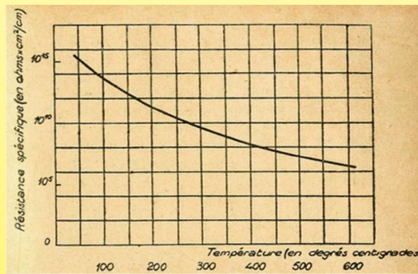
Variation of the specific resistance in ohms.cm/cm 2 of the porcelain according to the temperature (logarithmic curve). Between 20 °C and 300 °C its resistance is divided by 10,000 (1945 Matériaux électrotechniques modernes, Ultimheat Museum)
